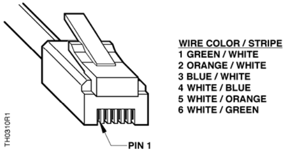
Figure 3. Terminating the RJ-11 Connector.
