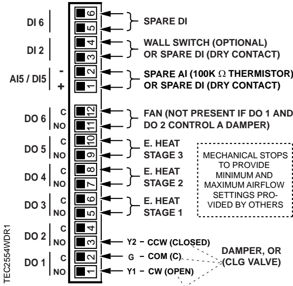
Figure 14. Application 2554 — Fan Coil Unit Cooling with Electric Heat.
