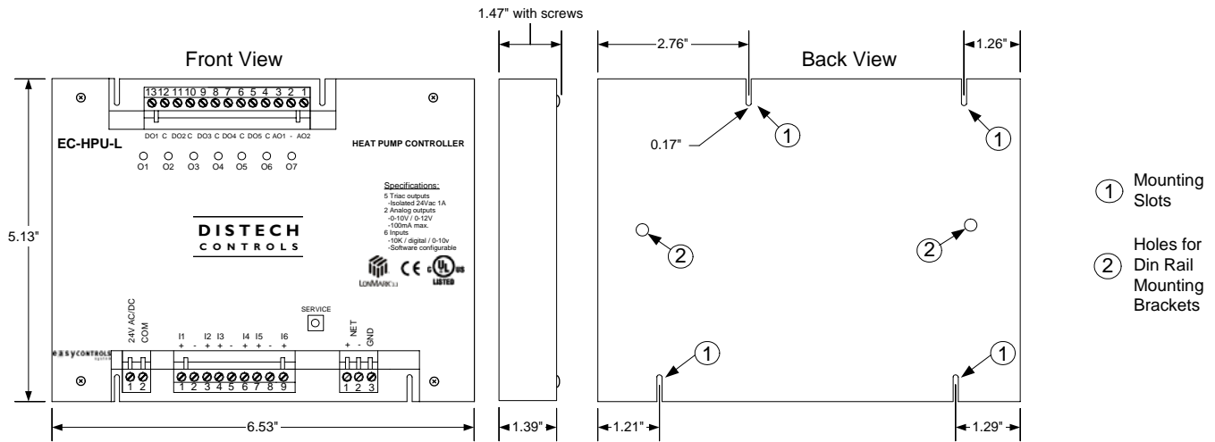
Figure 1: Controller dimensions and mounting options
